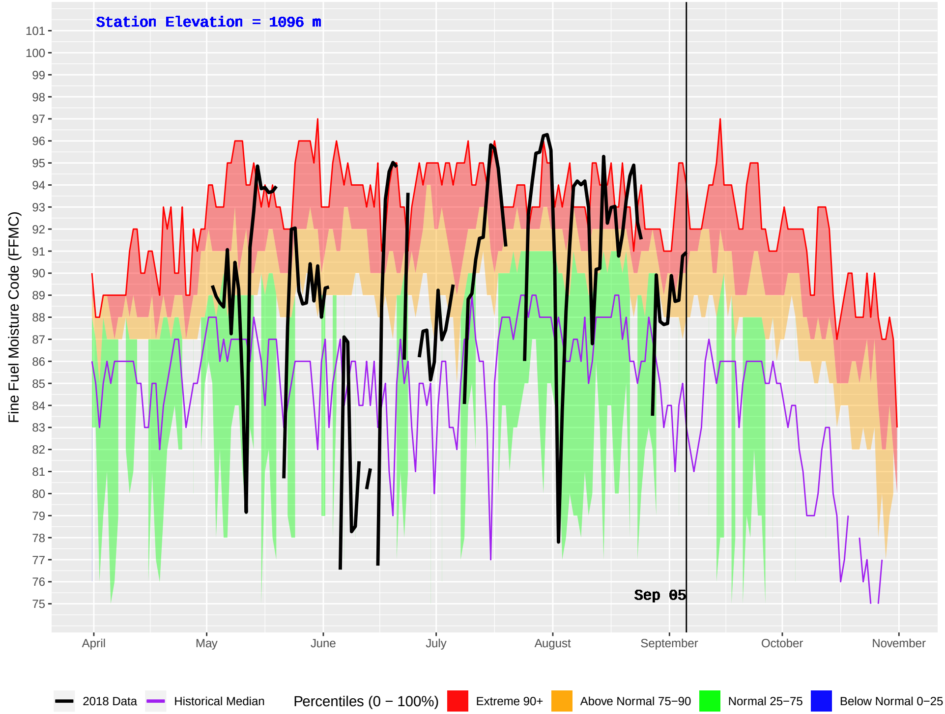
ANAHIM LAKE HUB (213) : Historical (1981–2016) and Current (2018) Daily Fine Fuel Moisture Code (FFMC)
