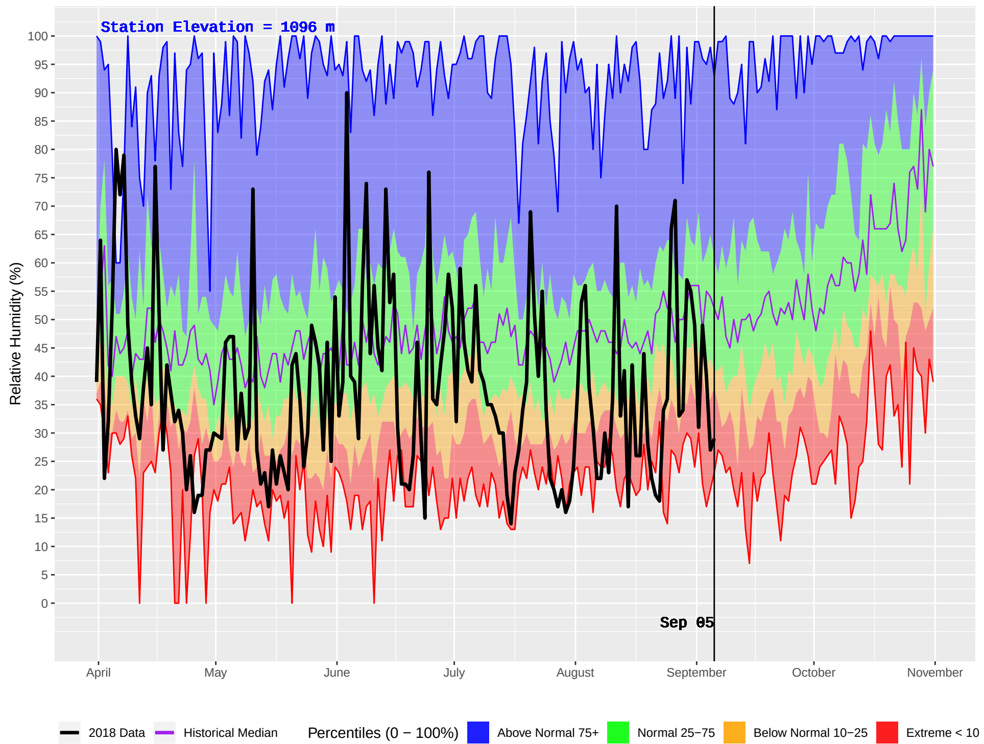
ANAHIM LAKE HUB (213) : Historical (1981–2016) and Current (2018) Daily Relative Humidity
