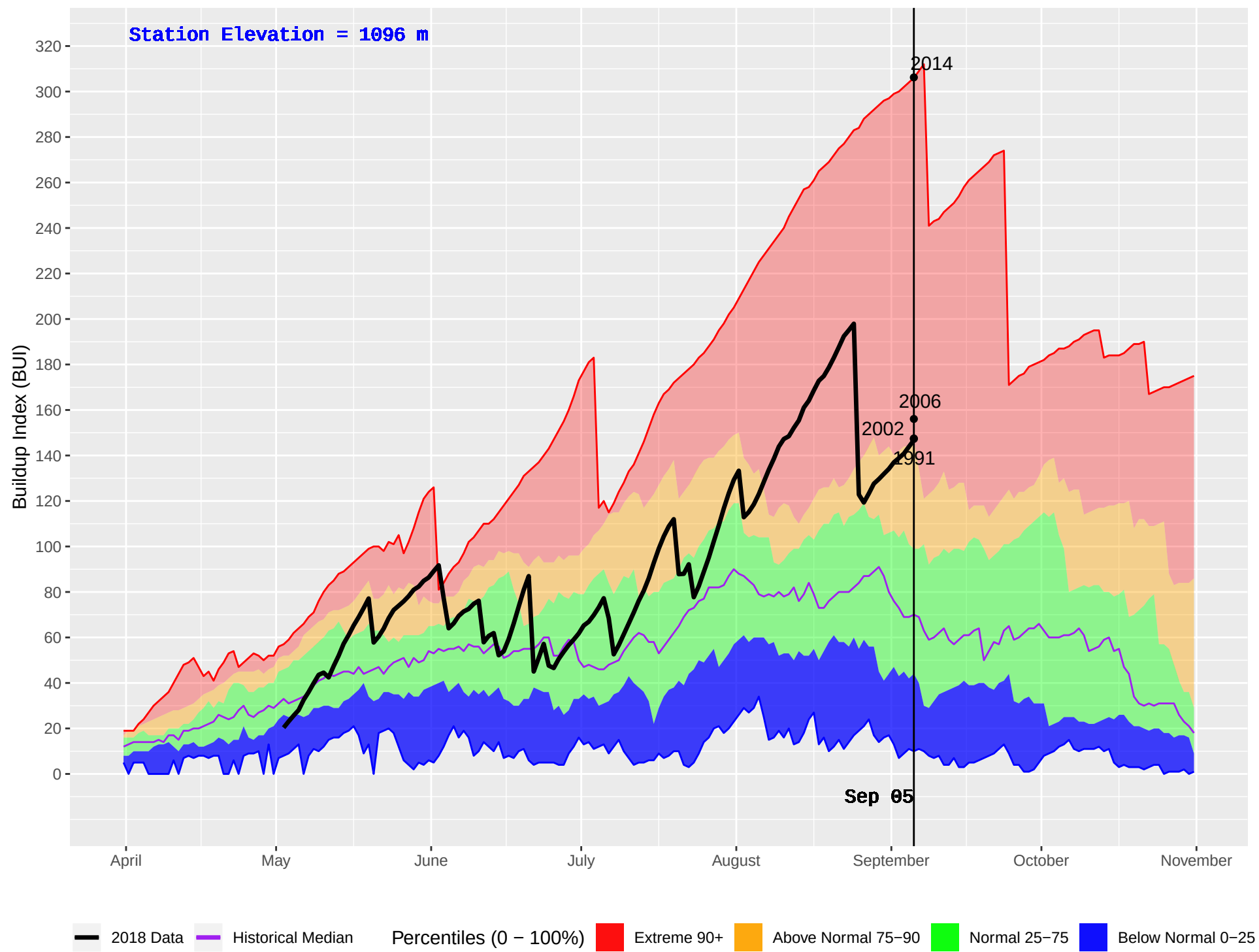
ANAHIM LAKE HUB (213) : Historical (1981–2016) and Current (2018) Daily Buildup Index (BUI)
